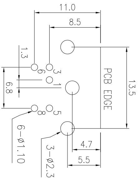
PCB LAYOUT (BOTTOM VIEW)
